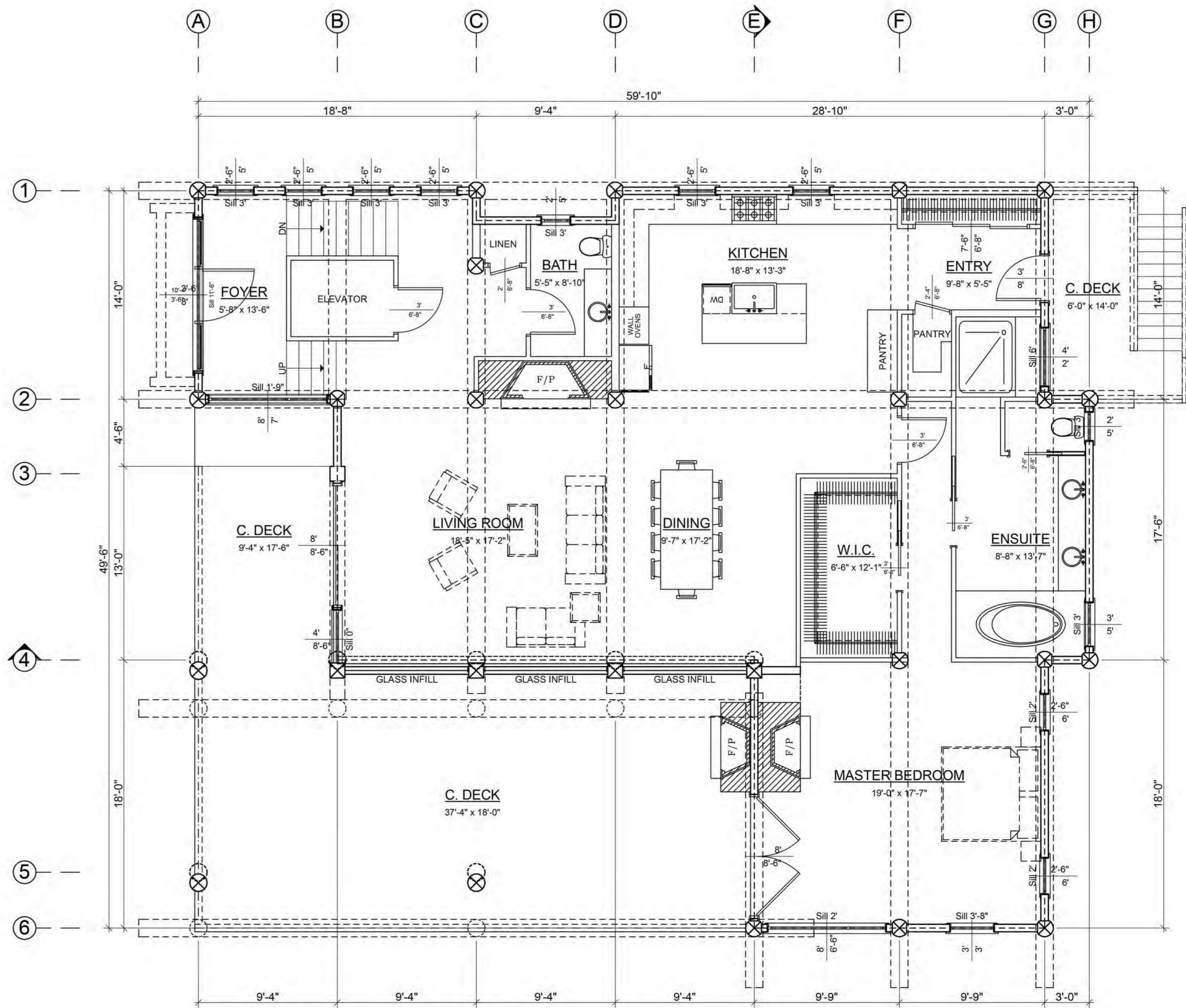
Sierra Blanca: FIRST FLOOR PLAN SCALE: 1/4" = 1'-0" AREA: 2068 sq ft
