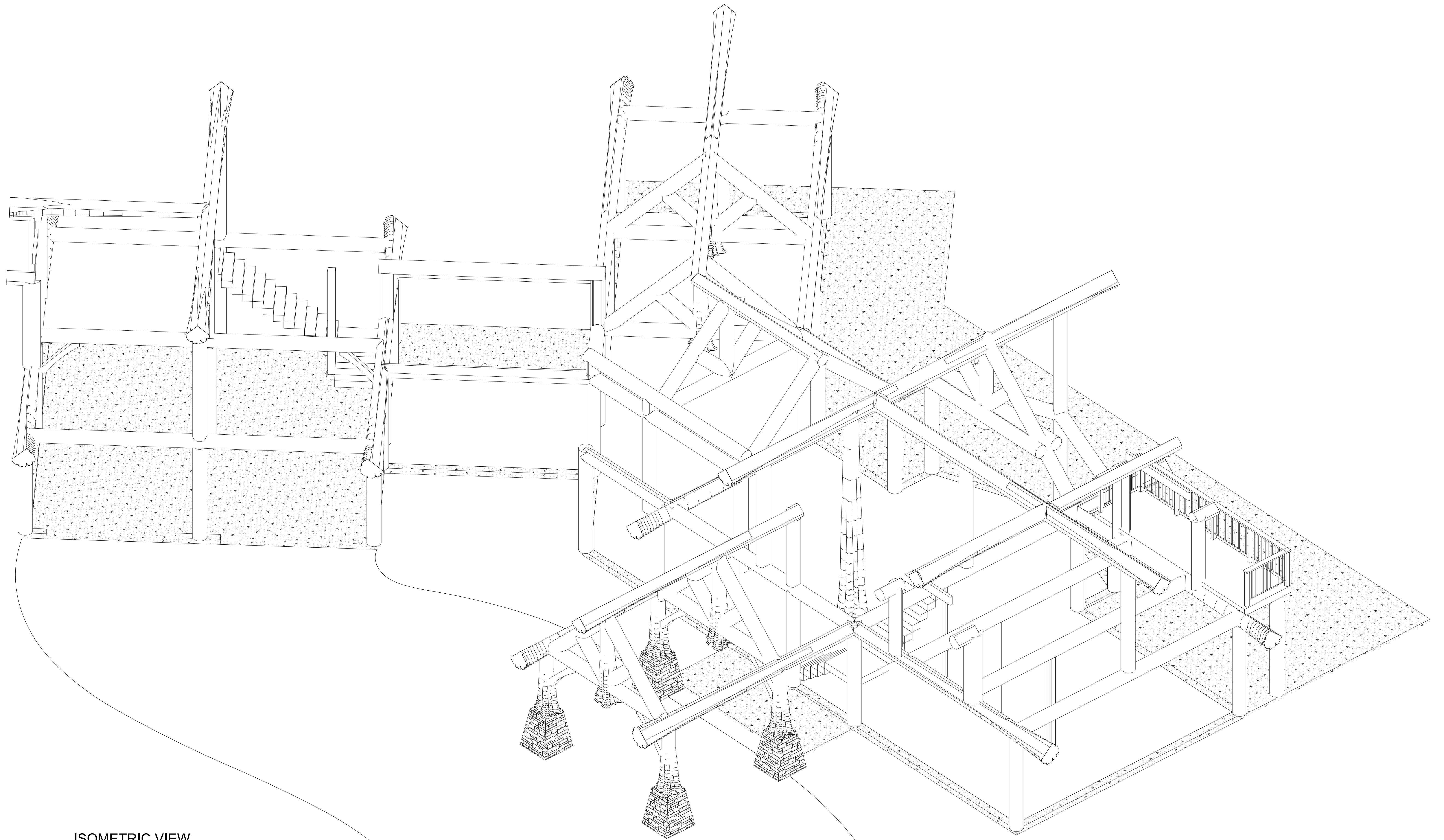
ISOMETRIC VIEW
