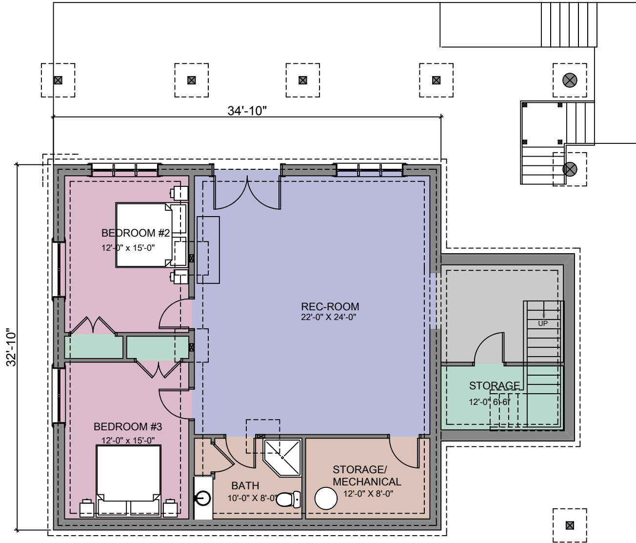
FOUNDATION PLAN W/ BASEMENT LAYOUT
