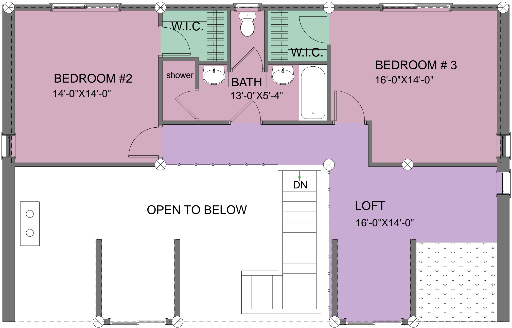
SECOND FLOOR PLAN AREA: 806 SQ. FT.
