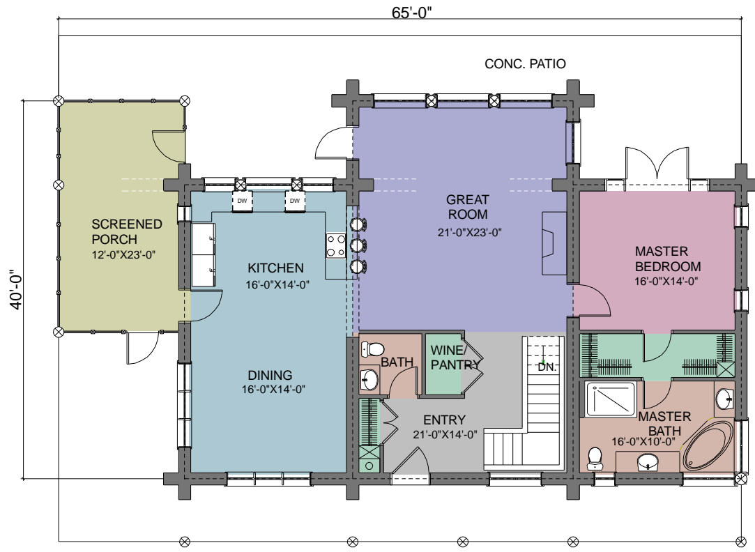
FIRST FLOOR PLAN AREA: 1697 SQ.FT.
