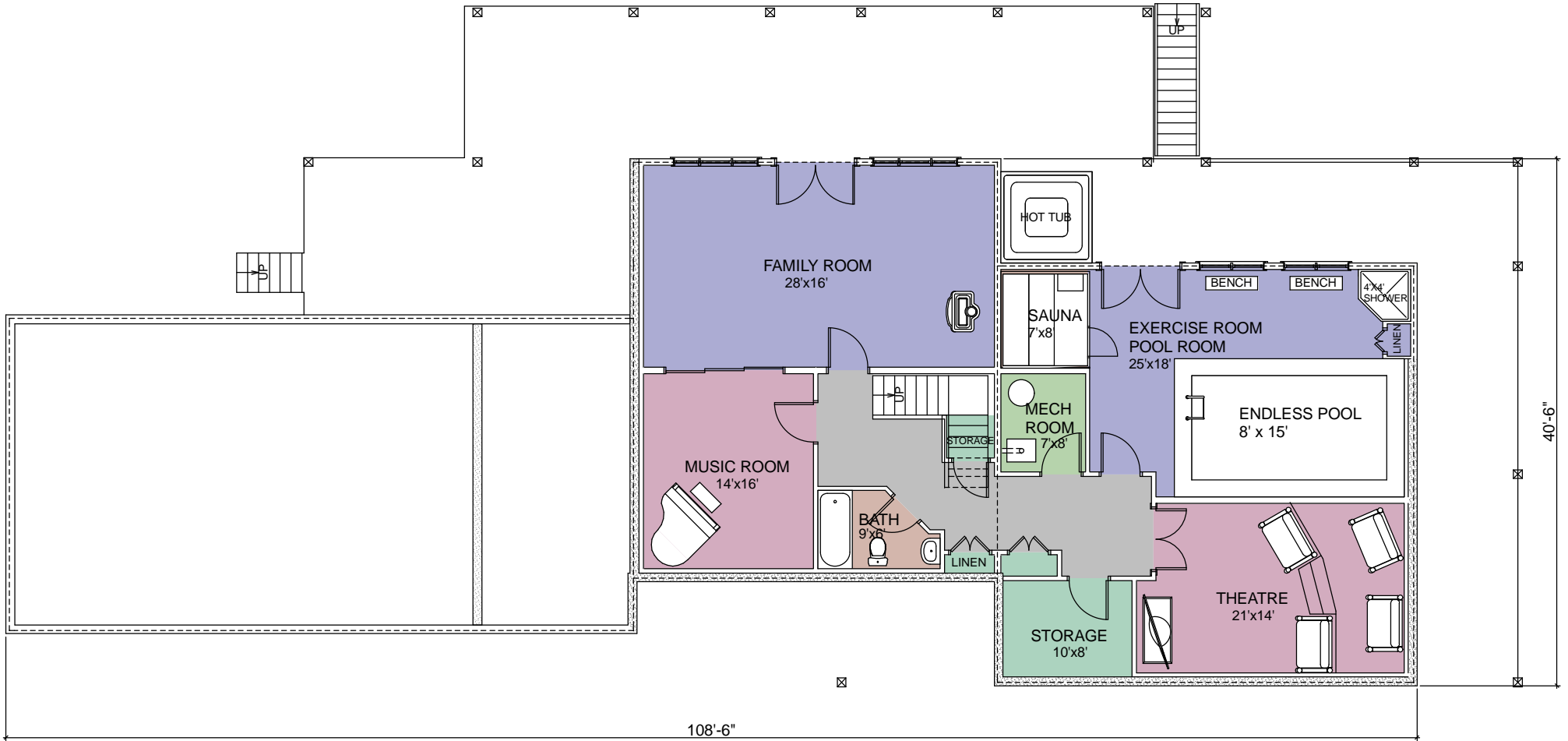
BASEMENT PLAN AREA: 1970 SQ. FT.
