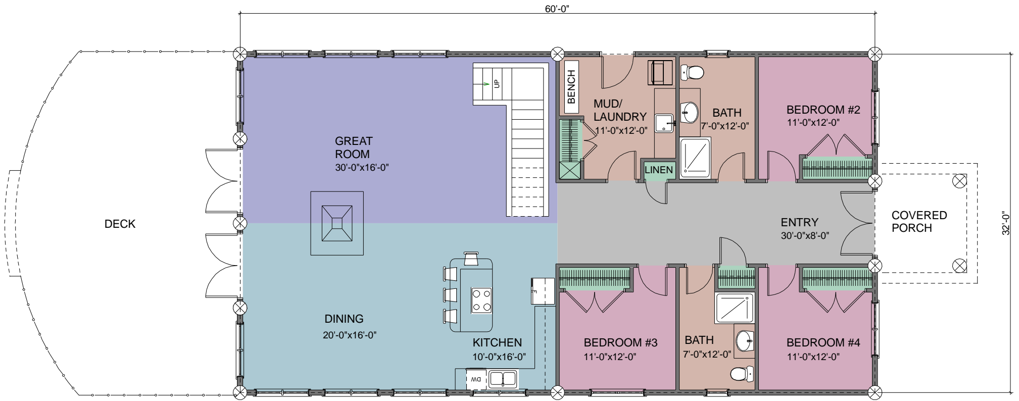
FIRST FLOOR PLAN AREA: 1970 SQ.FT.
