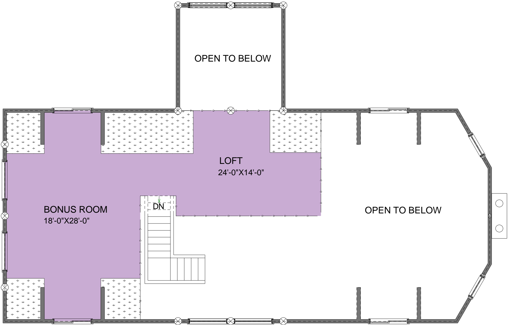
SECOND FLOOR PLAN AREA: 631 SQ. FT.
