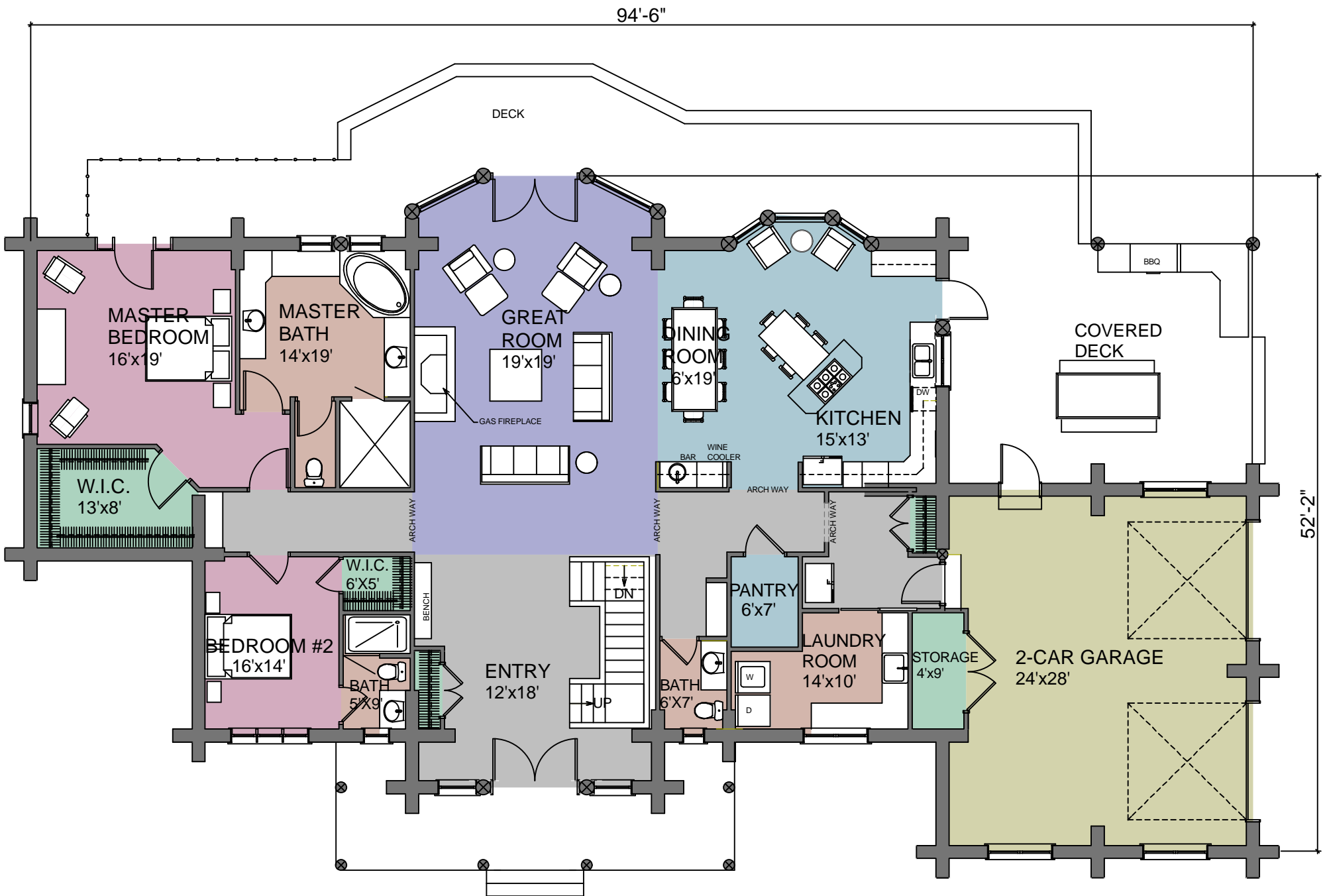
FIRST FLOOR PLAN AREA: 2688 SQ.FT.
