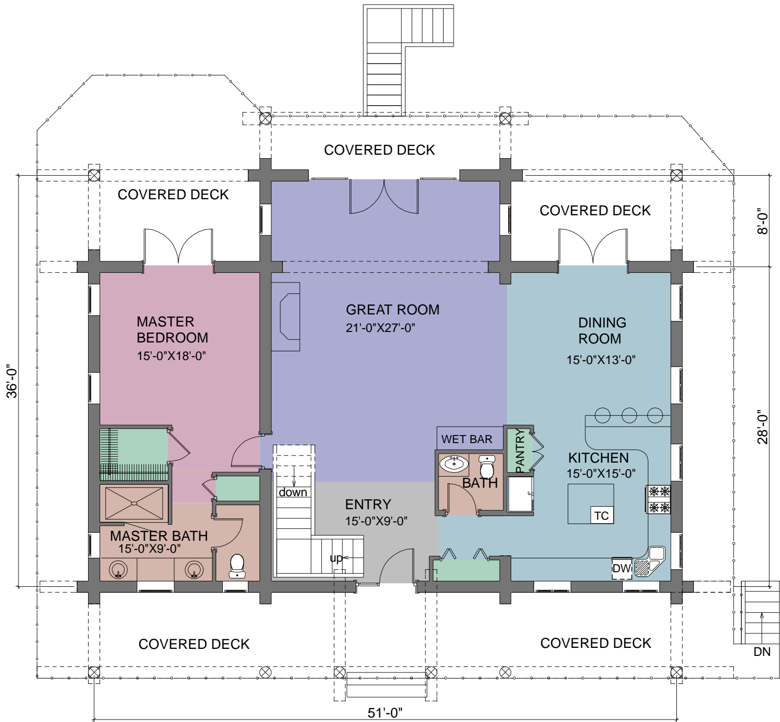
FIRST FLOOR PLAN AREA: 1640 SQ. FT.
