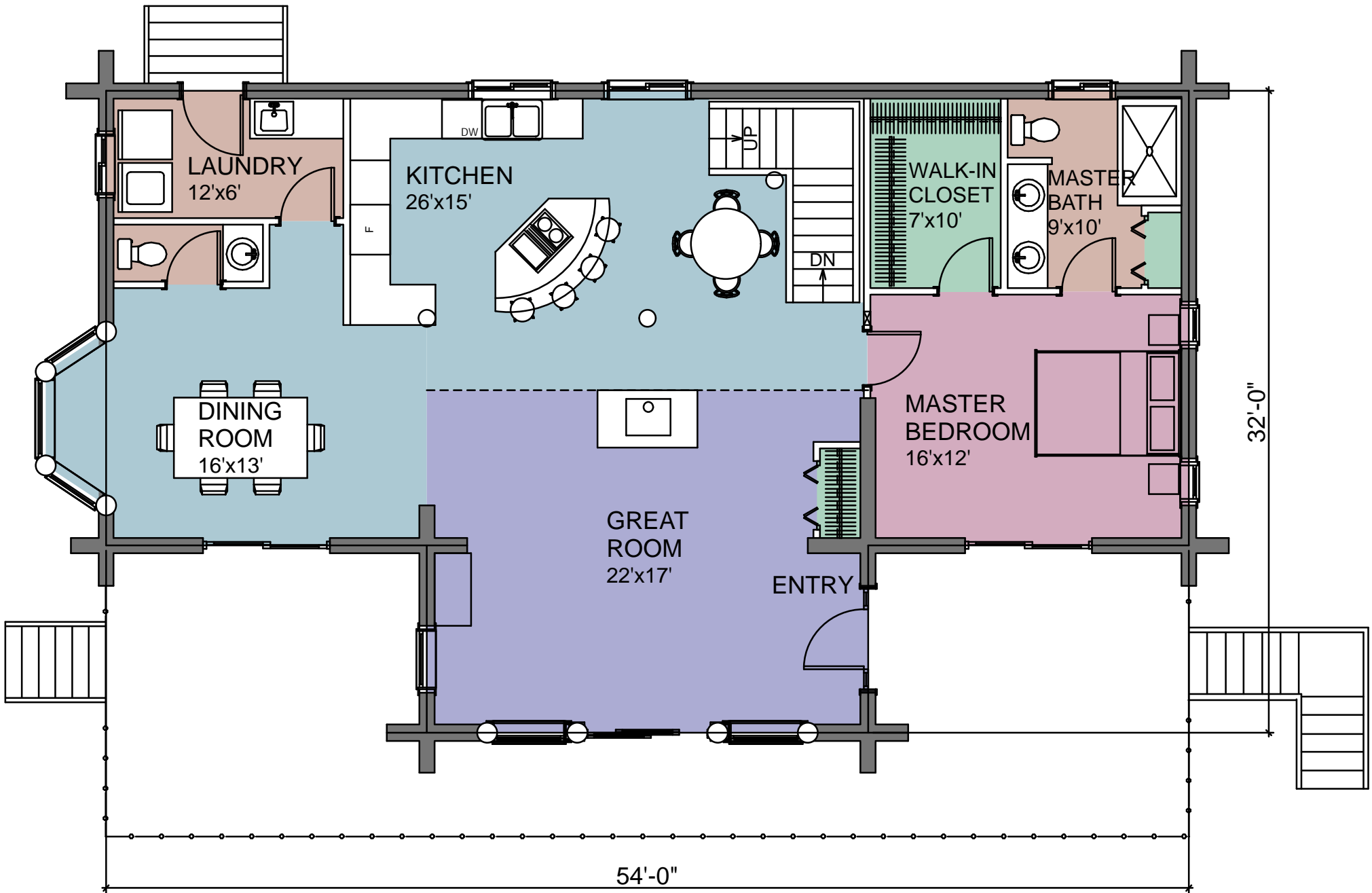
FIRST FLOOR PLAN AREA: 1529 SQ.FT
