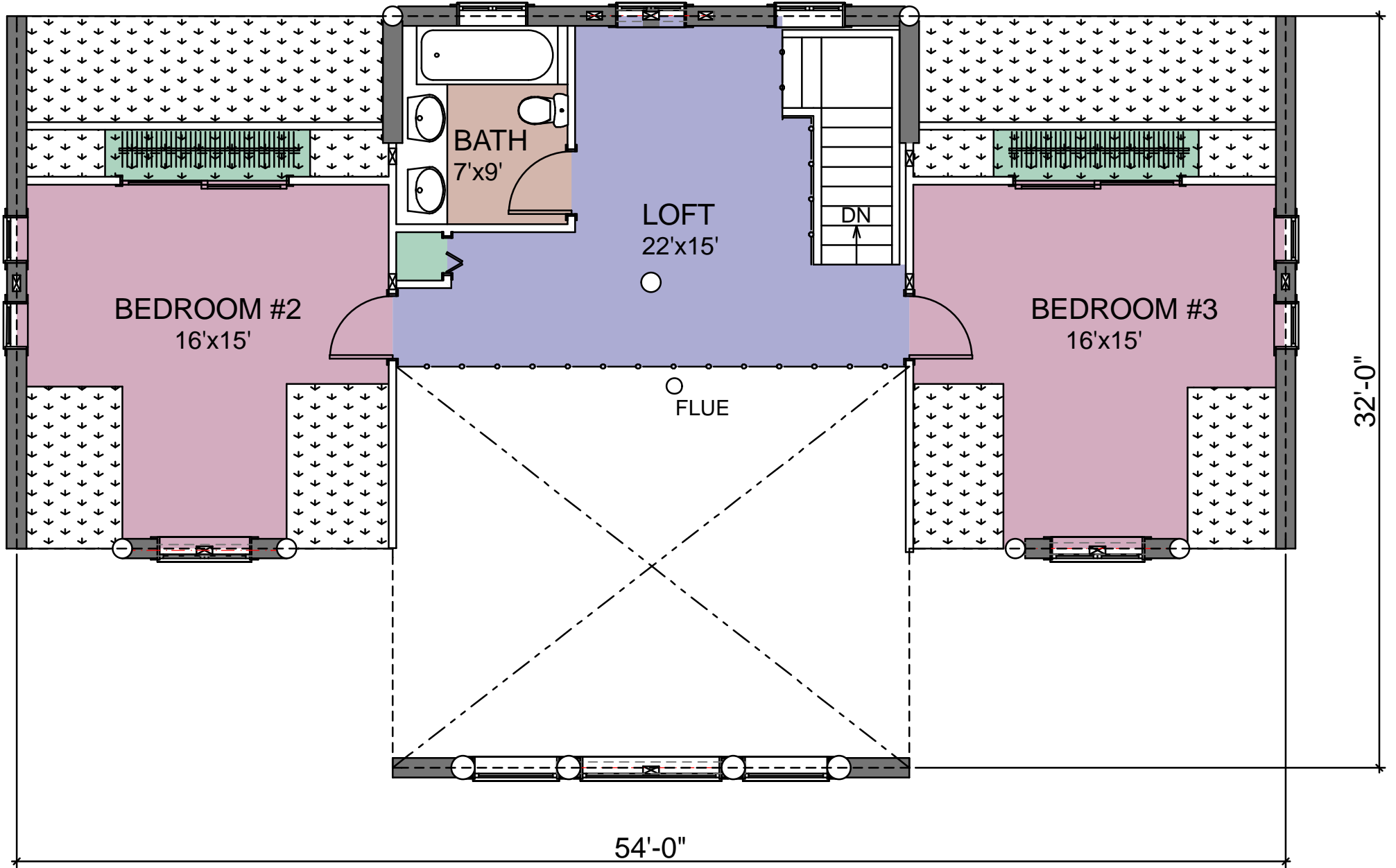
SECOND FLOOR PLAN AREA: 785 SQ. FT.
