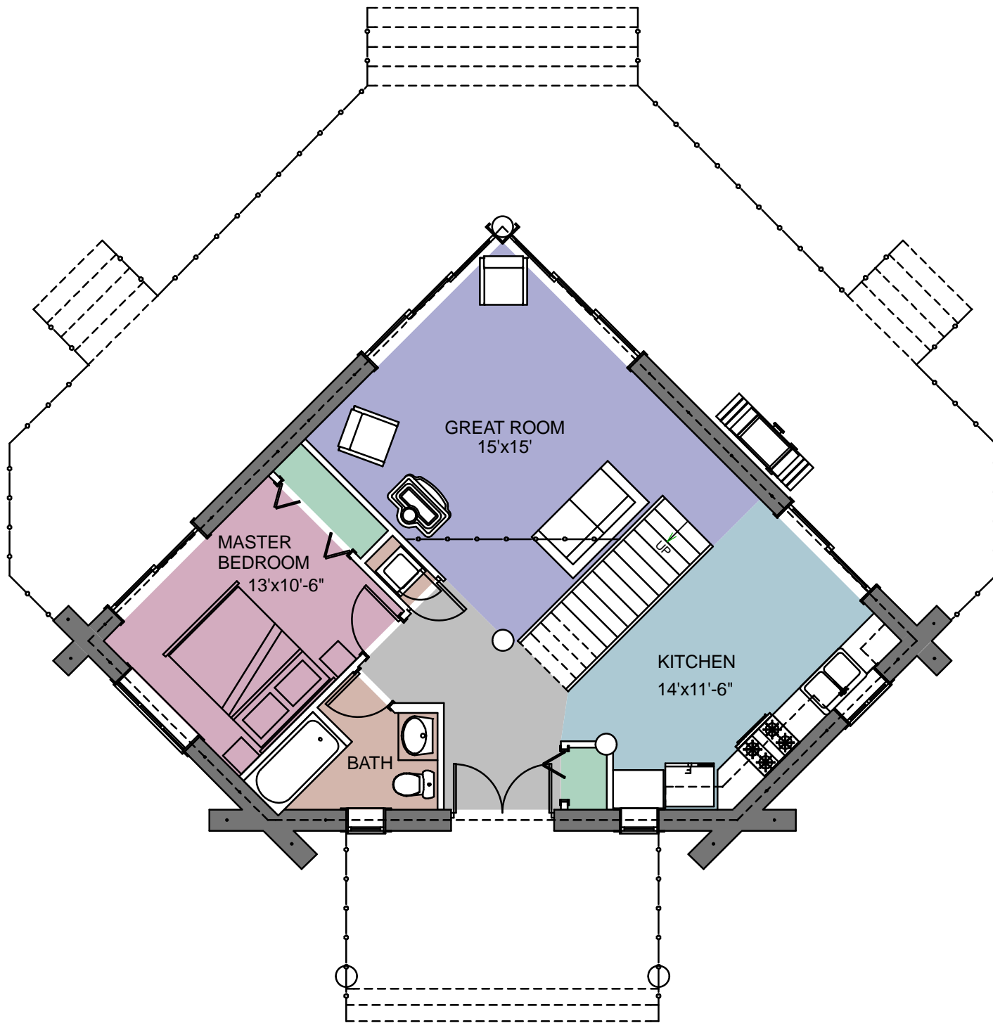
FIRST FLOOR PLAN AREA: 782 SQ. FT.
