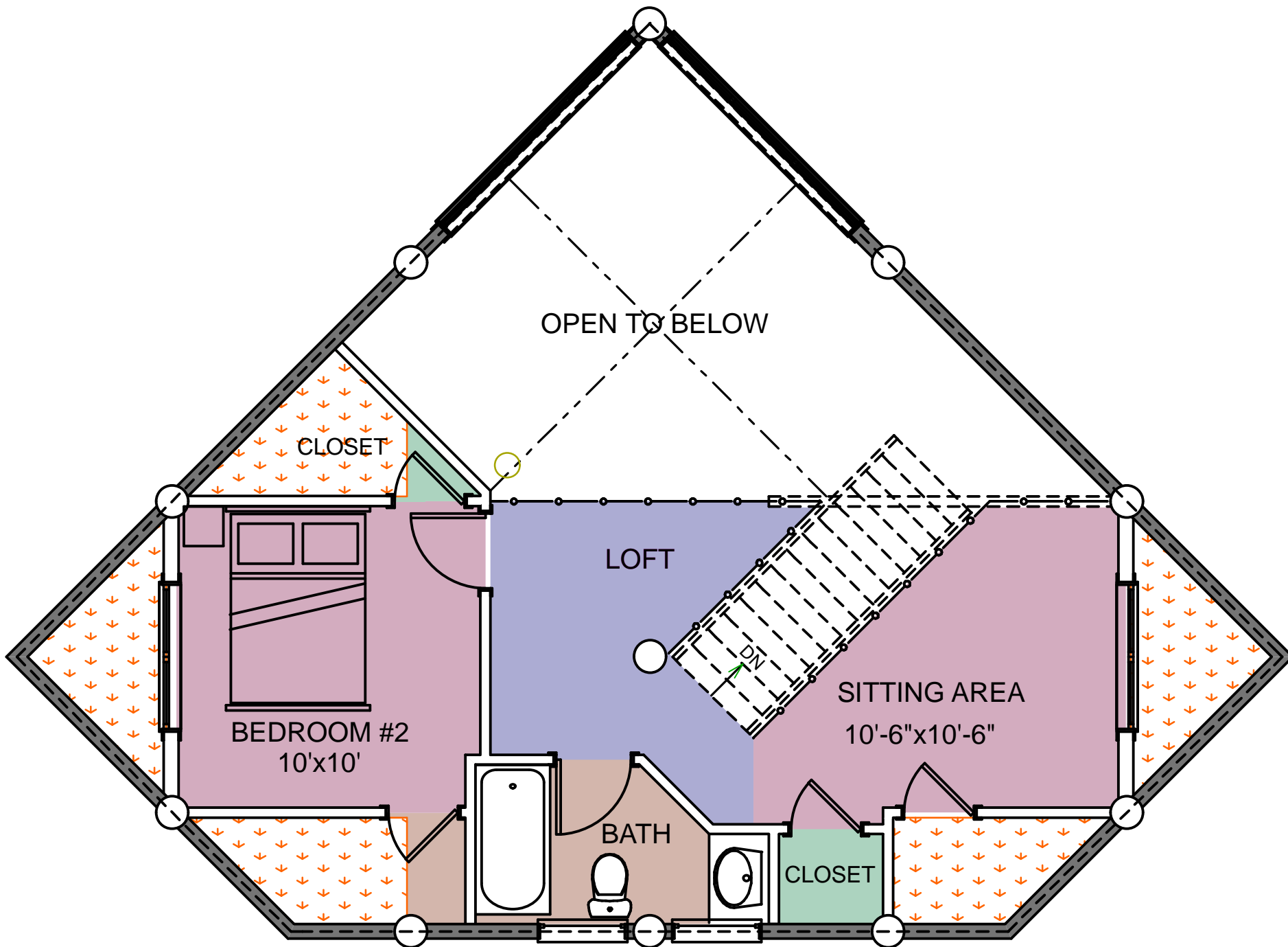
SECOND FLOOR PLAN AREA: 367 SQ. FT.
