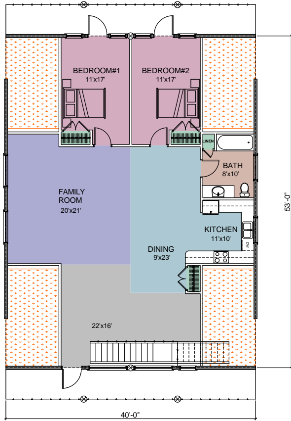
GARAGE SECOND FLOOR PLAN
