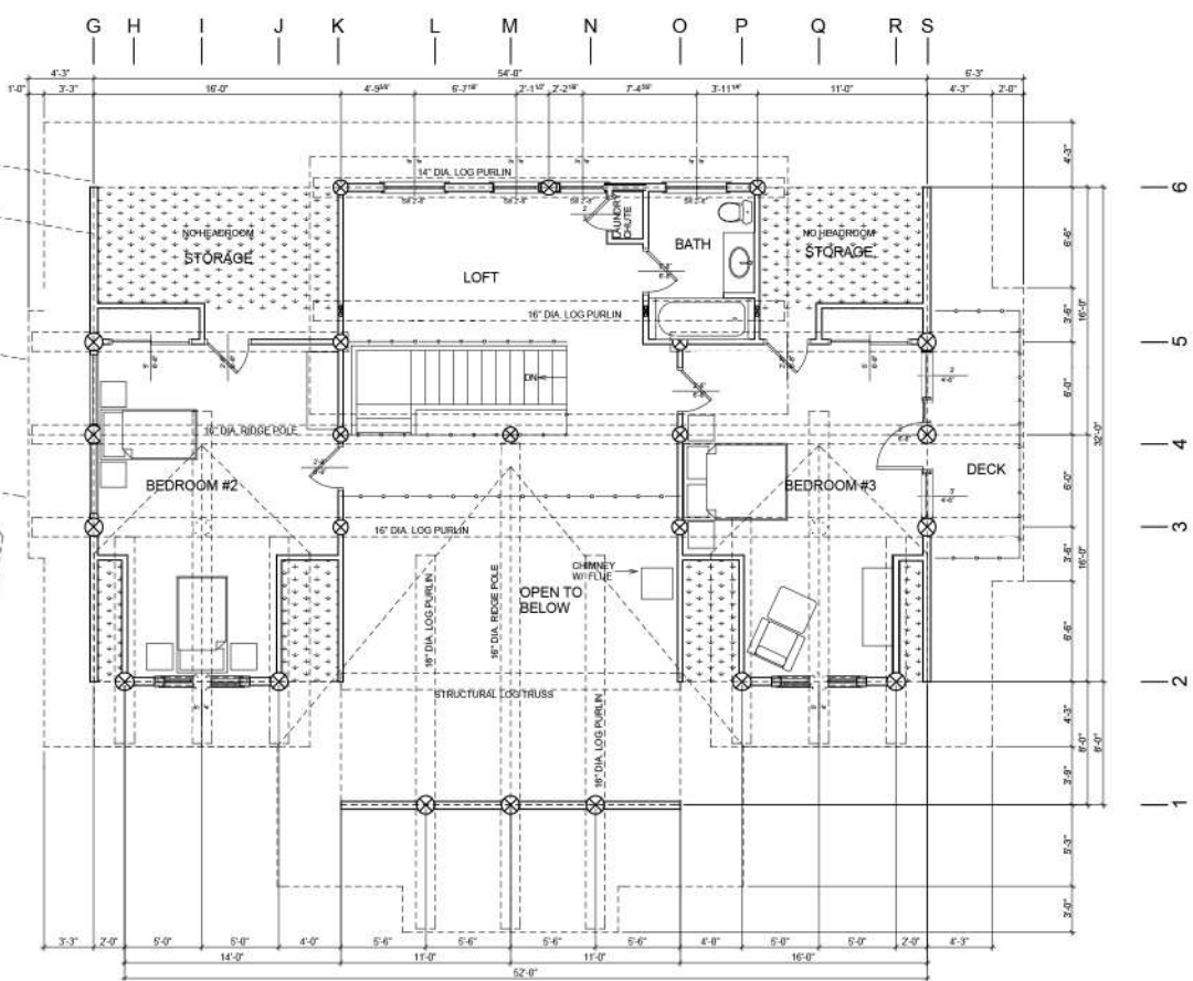
SECOND FLOOR PLAN AREA: 1169 SQ. FT.
