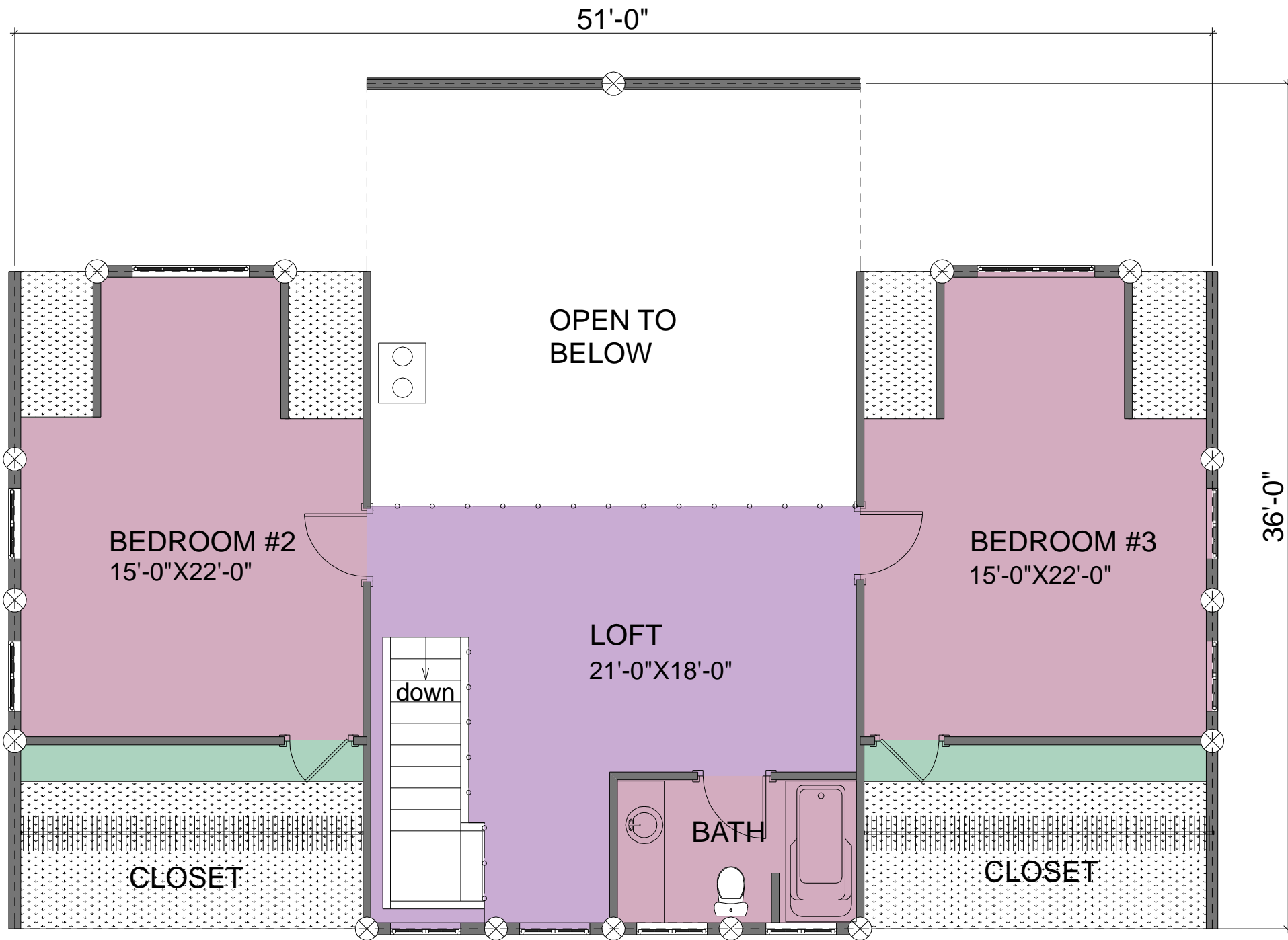
SECOND FLOOR PLAN AREA: 890 SQ. FT.
