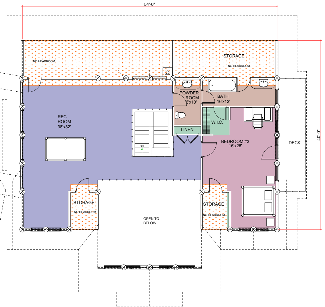
SECOND FLOOR PLAN AREA: 1260 SQ. FT.
